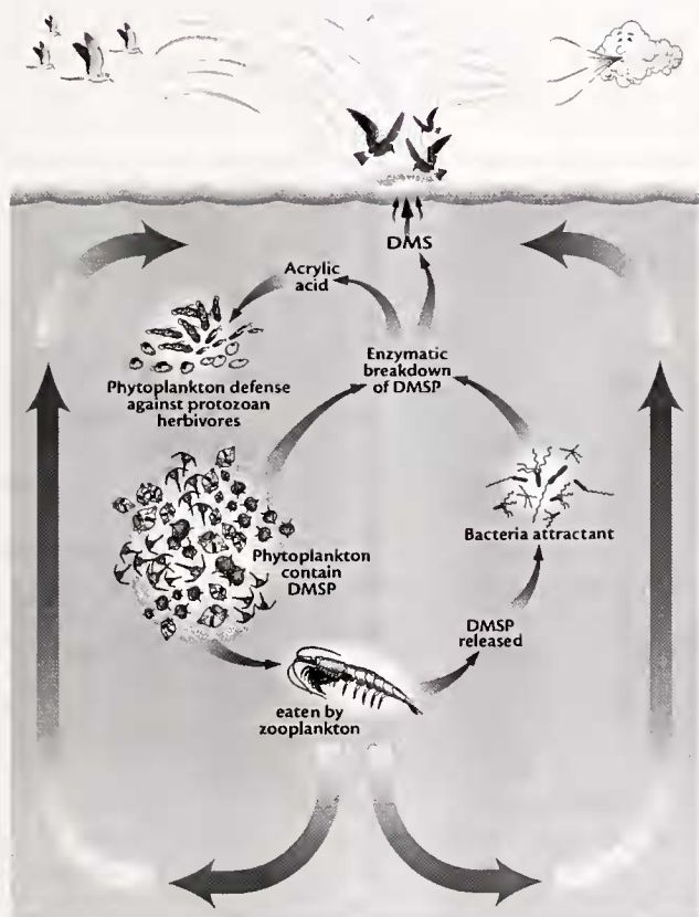
Figure 7. Diagram of the marine community that uses dimethylsulfoniopropionate (DMSP) and its breakdown products, dimethylsulfide (DMS) and acrylic acid, as chemical signals, at convergence zones in the open ocean.
